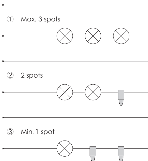
Connection Drawing
